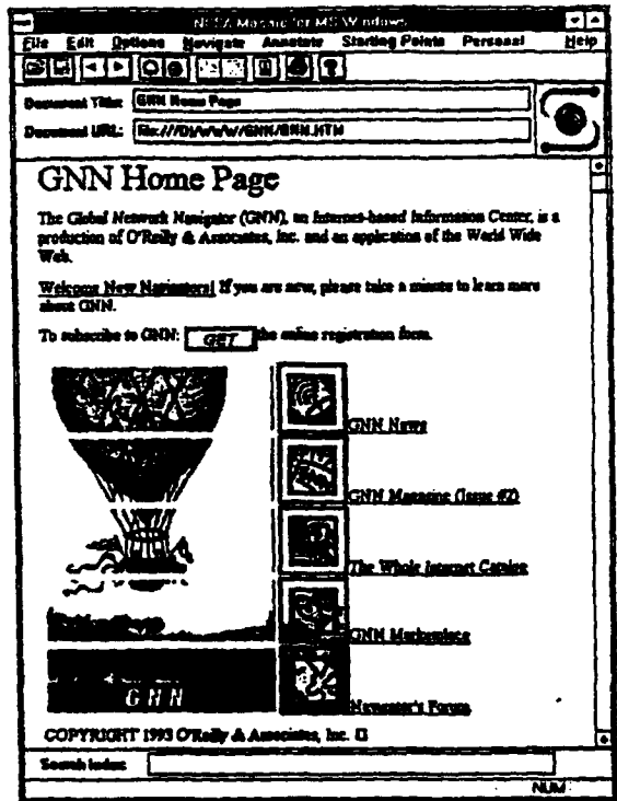
Figure 6: NCSA's Mosaic for Windows browsing O'Reilly's InfoCenter
